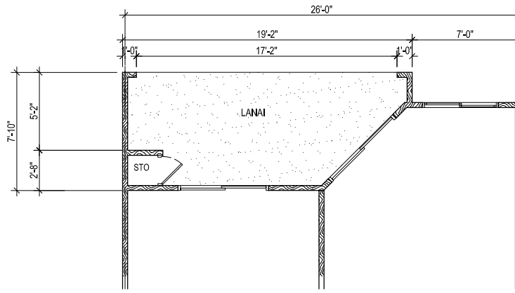
UNIT TYPE "B", TYPE "BR"(REVERSE) PARTIAL GROUND FLOOR PLAN
