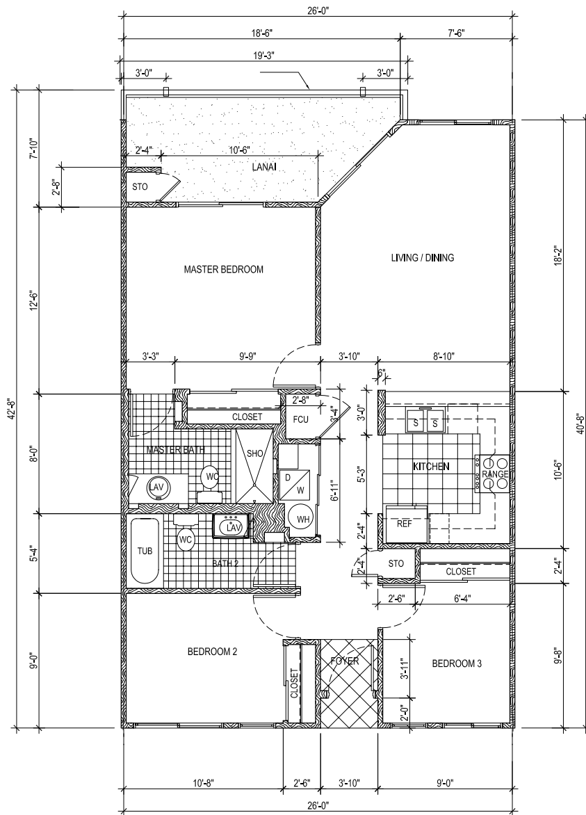
UNIT TYPE "B", TYPE "BR"(REVERSE) TYPICAL FLOOR PLAN
